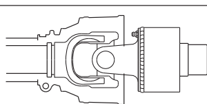
RUOTA LIBERA OVERRUNNING CLUTCH
